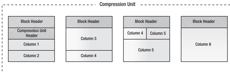
Figure 3-5. Layout of an HCC Compression Unit
