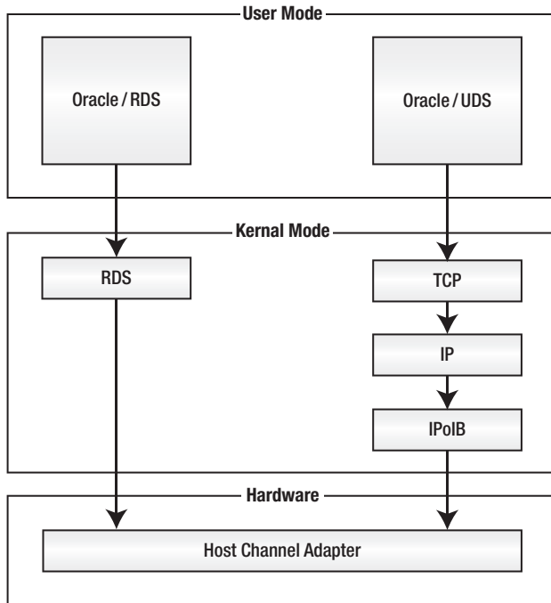
Figure 1-5. RDS schematic
