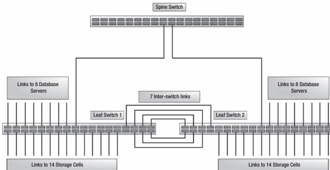
Figure 15-4. An Exadata full rack InfiniBand network
